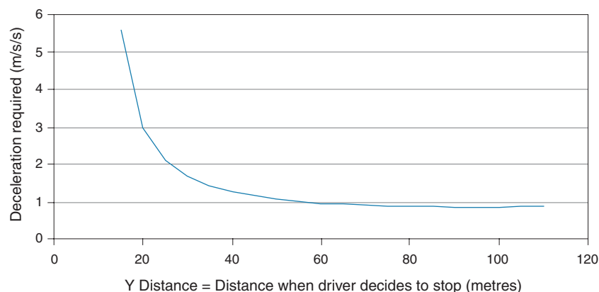
Figure 6.4 Deceleration rate required by second vehicle to stop if seeing first vehicle at 'Y-distance' metres from junction
