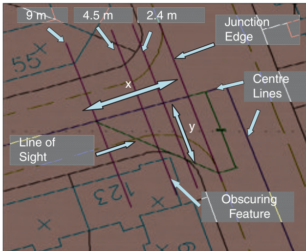
Figure 3.2 Y-distance at junctions
