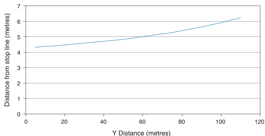
Figure 6.3 Distance at which first vehicle must see second vehicle in order to stop
