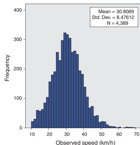
Figure 5.1b Link speeds
