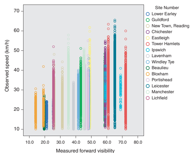
Figure 4.7 Speed ATC data for links
