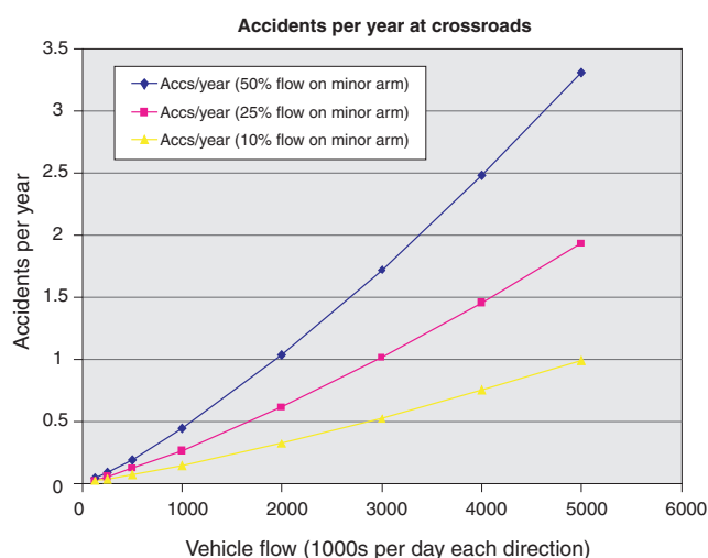
Figure 10.3 Effect of varying major and minor flows on accidents per year predicted by SafeNet
