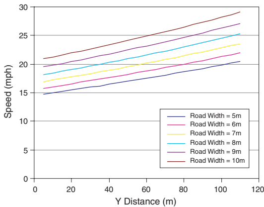
Figure 5.5 Junction model – manual speeds with average site features (non-turners only)
