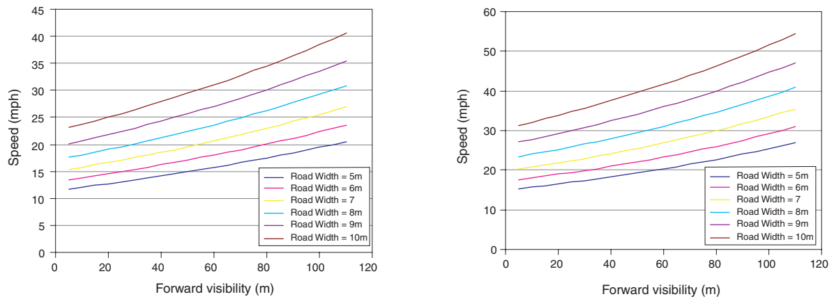
Figure 5.2 Link model – manual speeds with average site features
