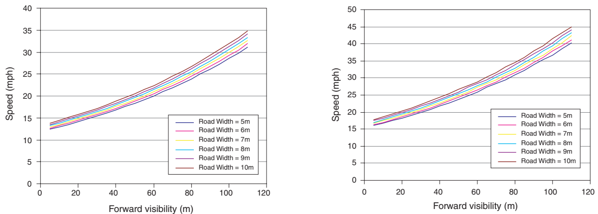
Figure 5.3 Link model – ATC speeds
