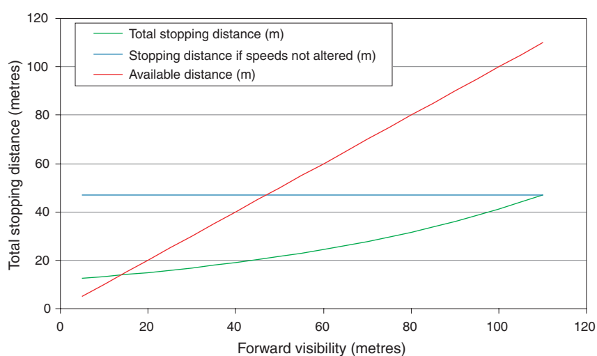
Figure 6.2 Modelled stopping distances on a link of width 9 metres
