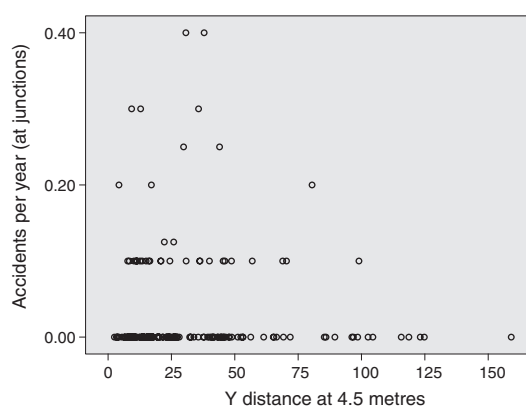
Figure 7.4 Junction accidents – according to Y-distance
