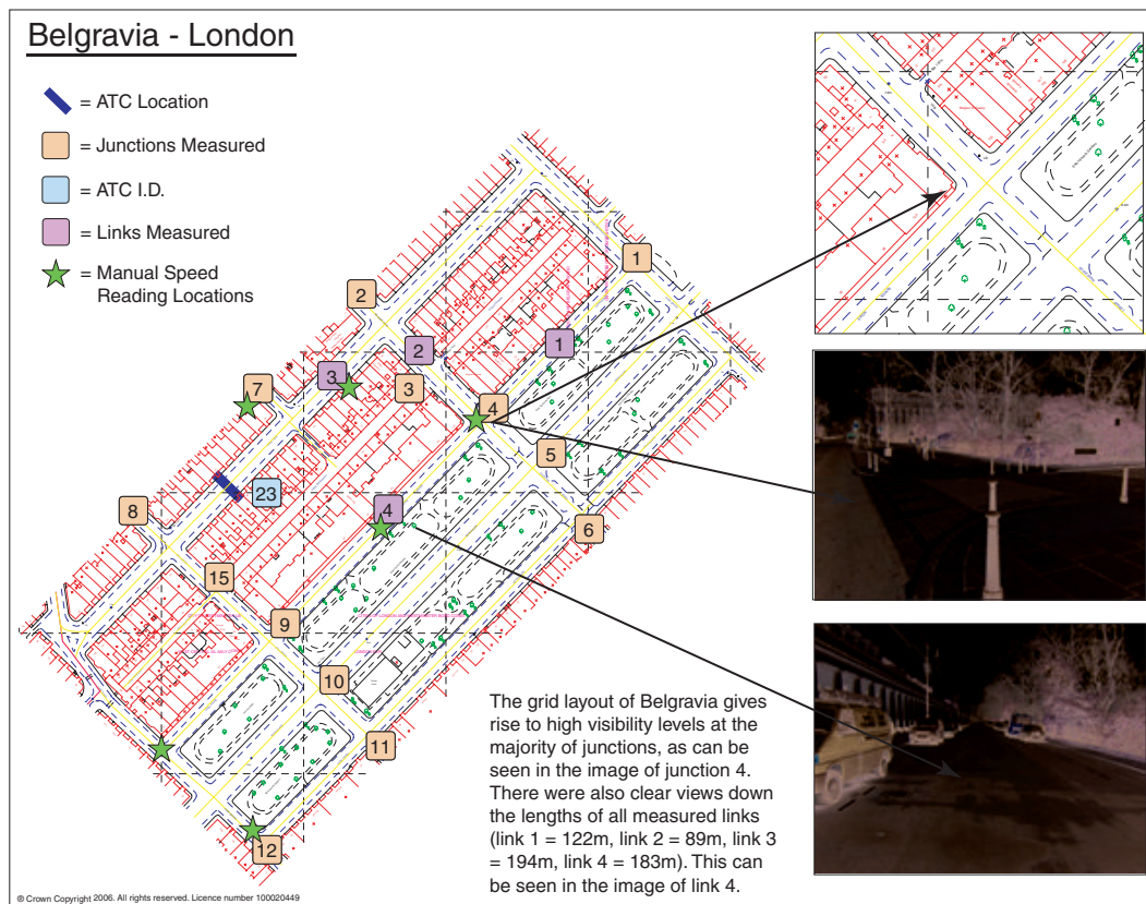
Figure 4.5 Belgravia – grid layout (large visibilities)
