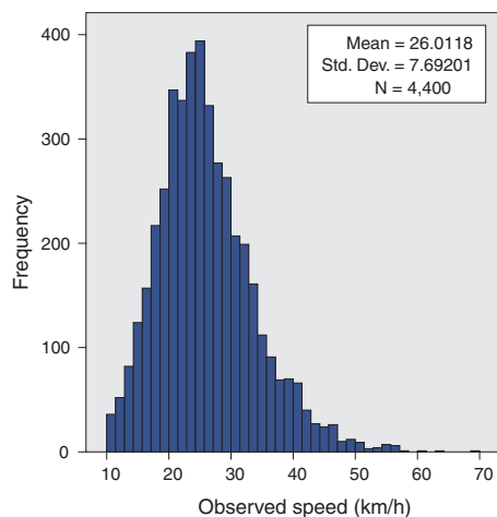
Figure 5.1a Junction speeds
