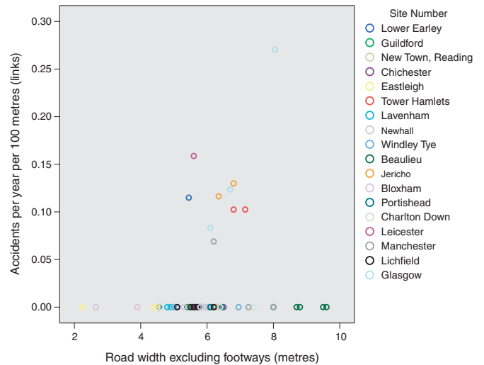
Figure 7.8 Link accidents per 100 m – according to road width
