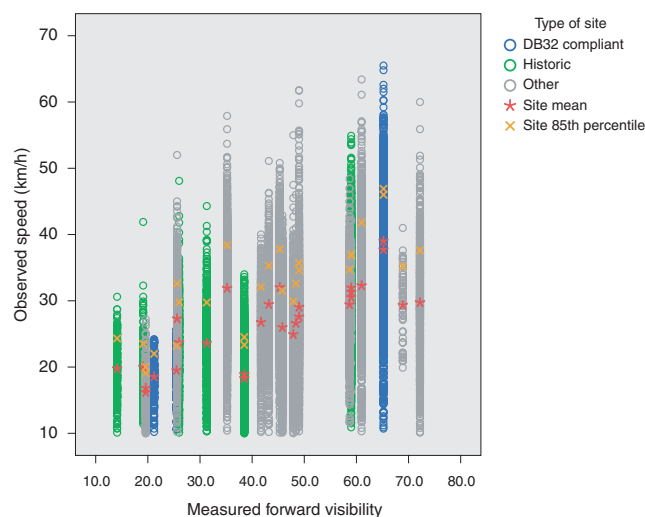
Figure 4.6 Speed ATC data for links (by site type)
