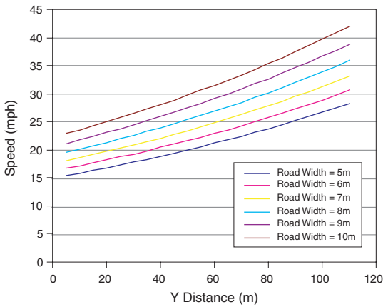
Figure 5.6 Junction model – ATC speeds
