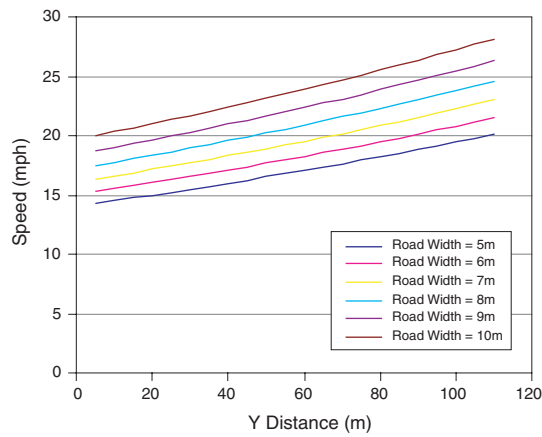
Figure 5.4 Junction model – manual speeds with average site features (all vehicles)
