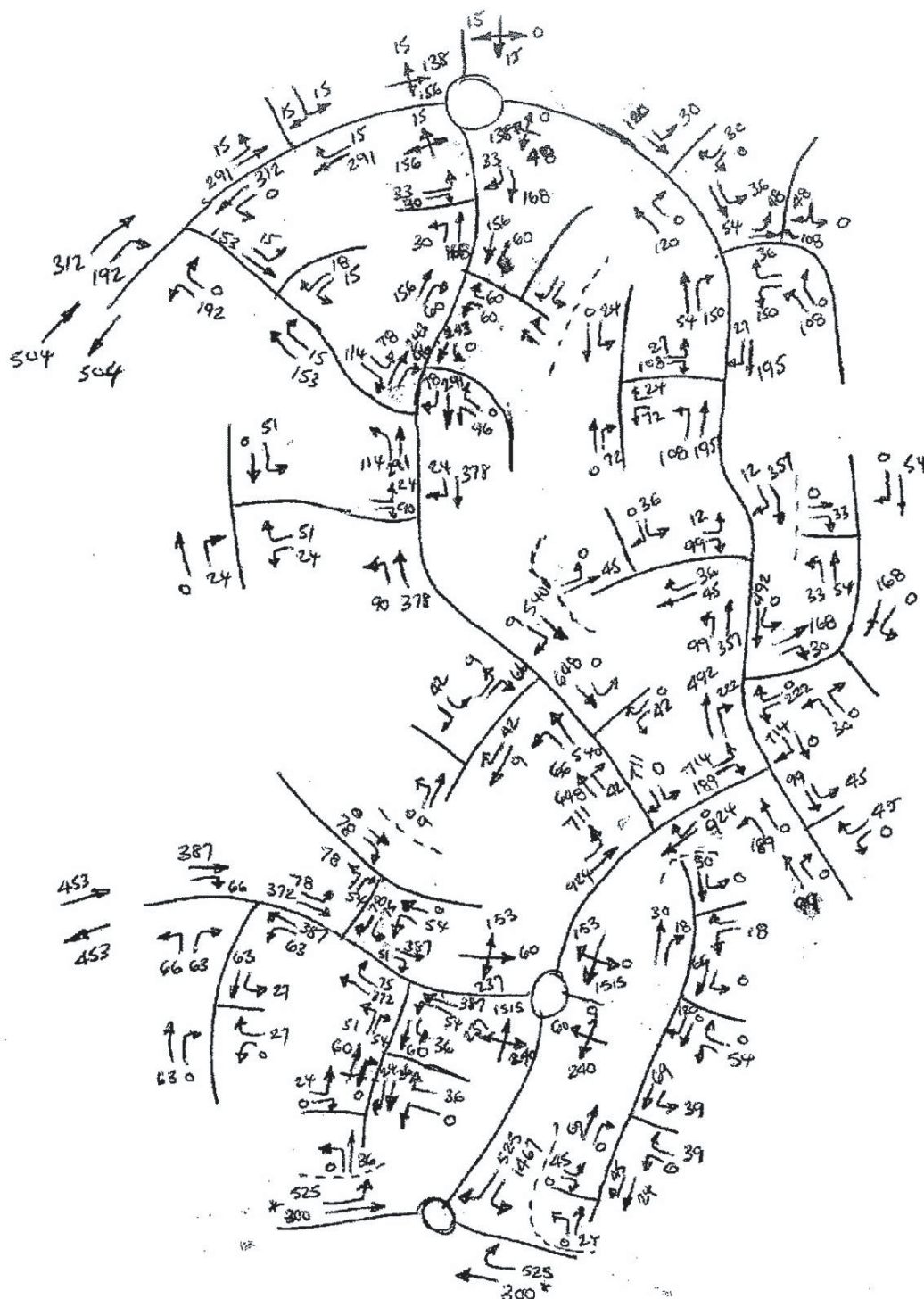
Figure 10.1 DB32 network for SafeNet analysis
