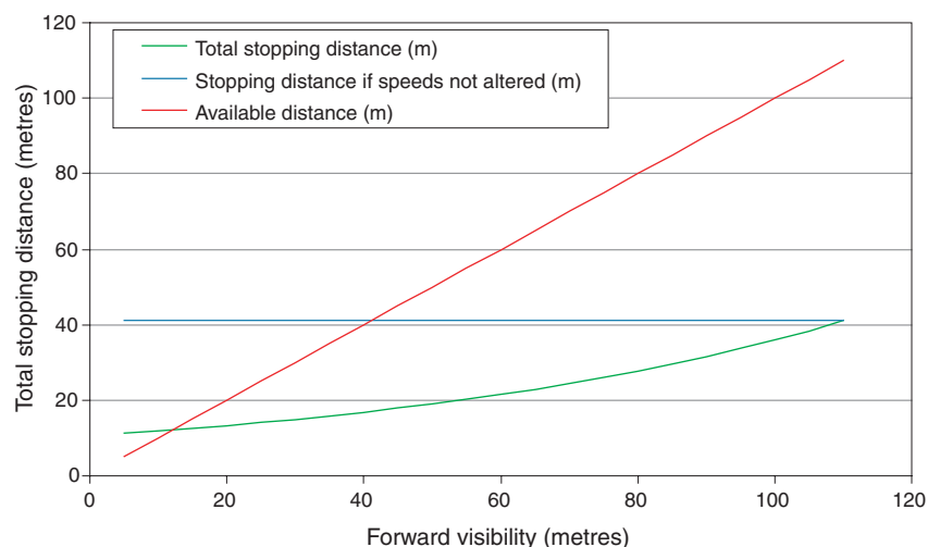
Figure 6.1 Modelled stopping distances on a link of width 5 metres
