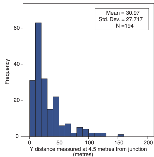
Figure 4.3 Range of observed junction visibilities
