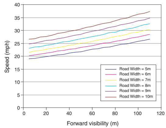
Figure 5.4 Junction model – manual speeds with average site features (all vehicles)
